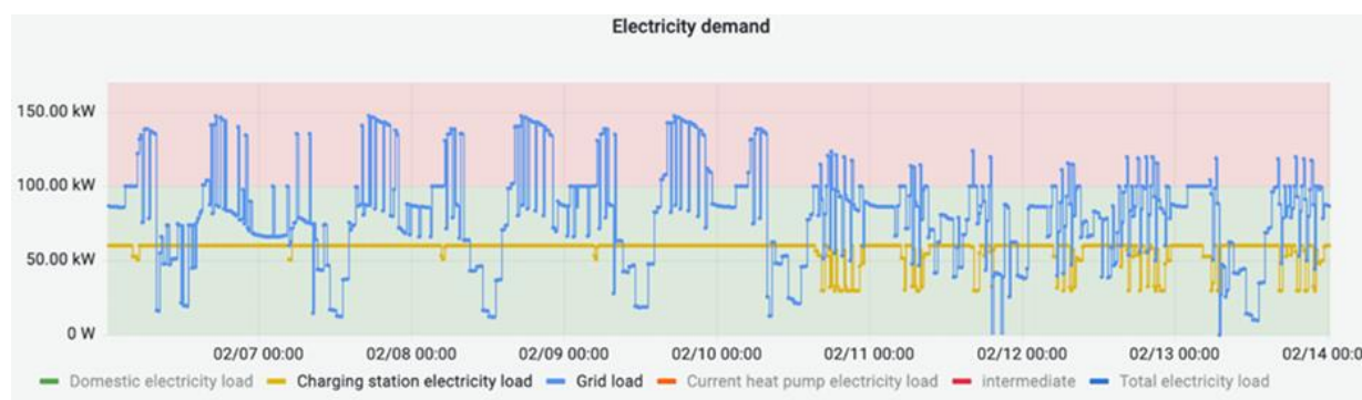
Figure 13: Example of Peak Shaving above 100kW Threshold on the Collective Load Curve (DuCoop EAN)
