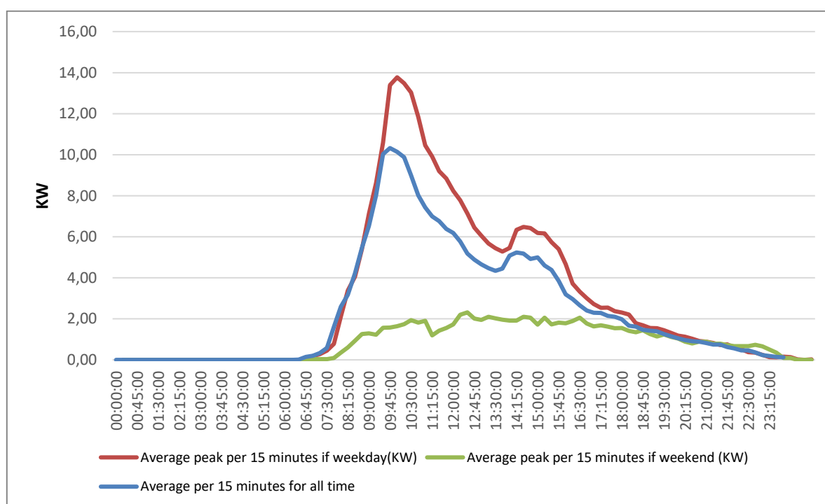
Figure 48: Average Peak Value per 15 Minutes
