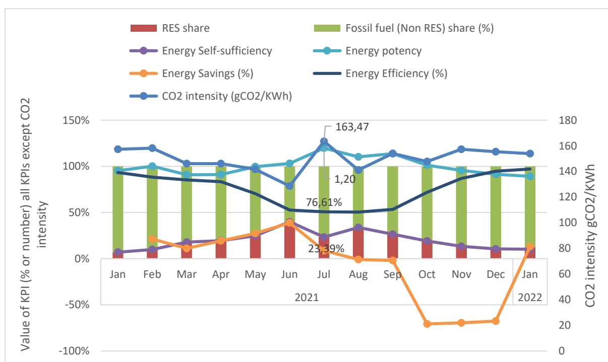
Figure 3: Monthly Technical Heat KPIs Graph (namely Renewable Energy Sources Share, Fossil Fuel (Non-RES) Share, Energy Self-sufficiency indicator, Energy Potency, Energy Savings, Energy Efficiency, and CO 2 intensity) Calculated based on Real Data for the Heat Network
